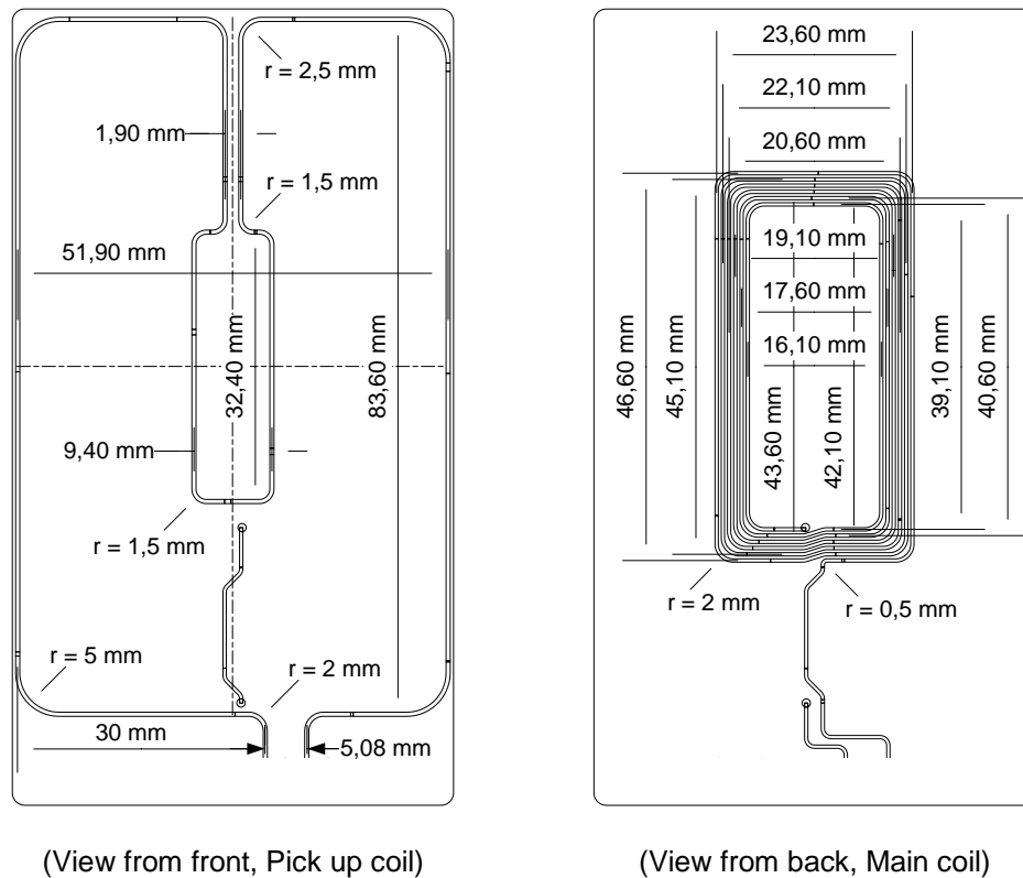
Figure D.4 — Reference PICC 4 Pick up coil and Main coil layouts
