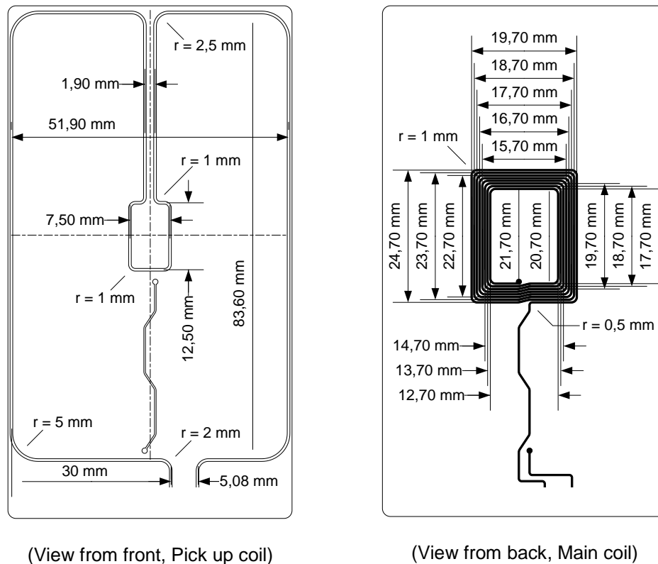
Figure D.6 — Reference PICC 6 Pick up coil and Main coil layouts
