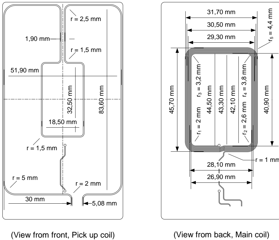
Figure D.3 — Reference PICC 3 Pick up coil and Main coil layouts
